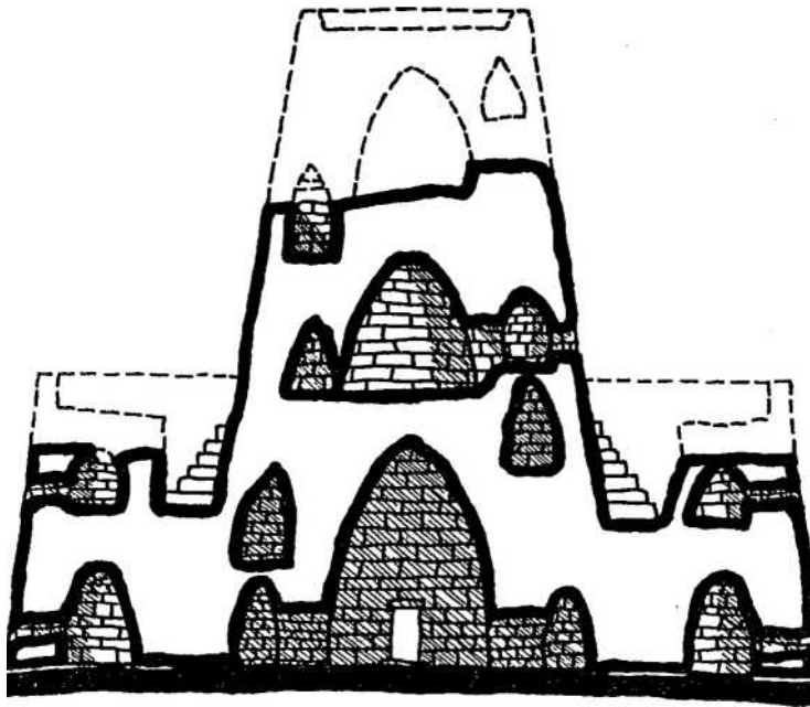
Ouragh of San Antine. Schematic section
