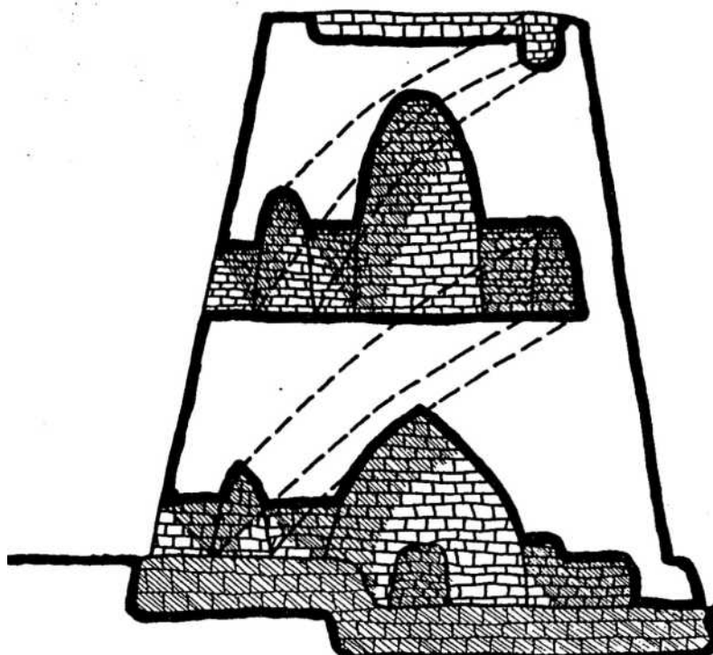
Nuragha of Silanus. Chopped off.
